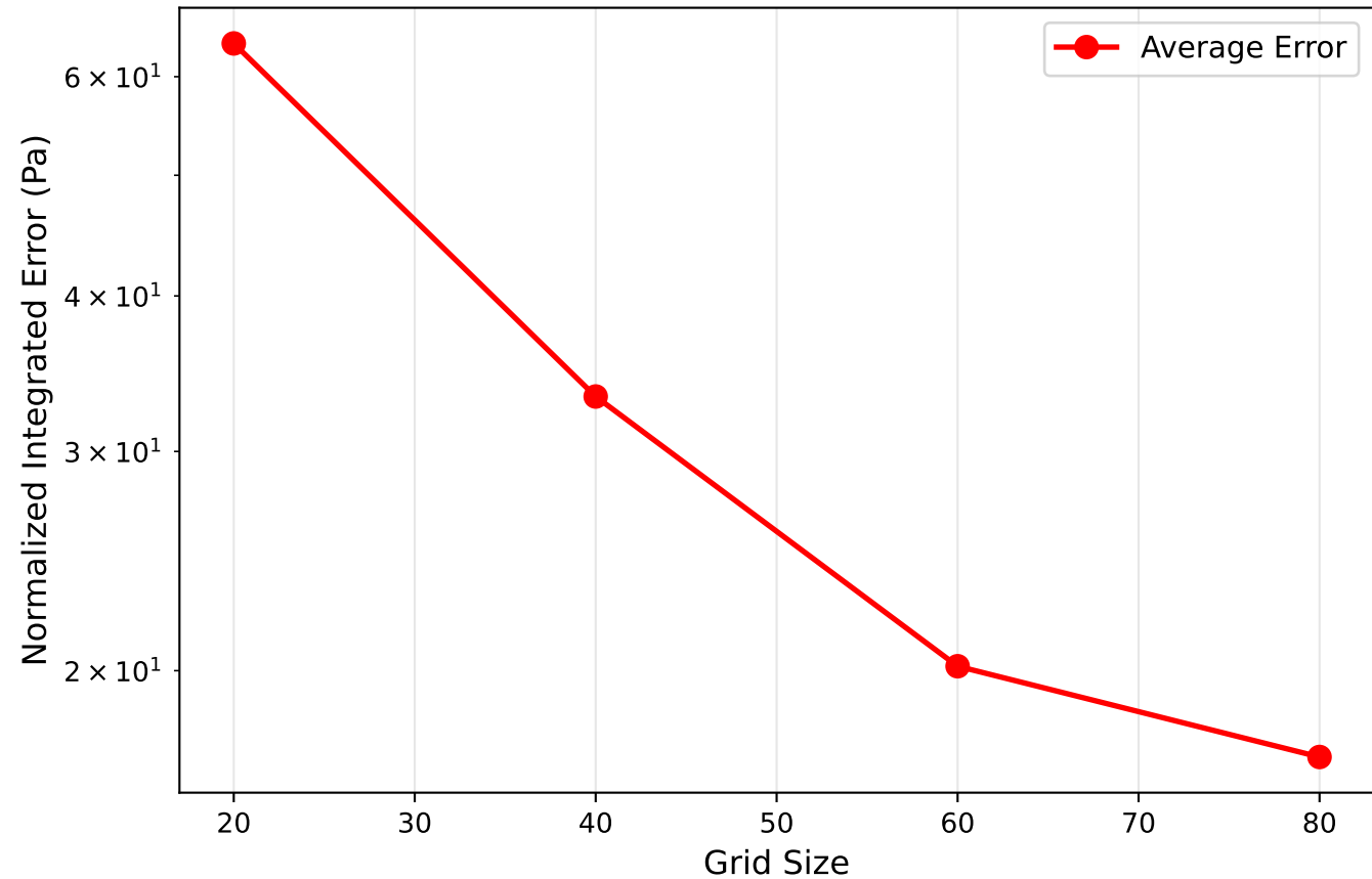
Total Normalized Integrated Error
