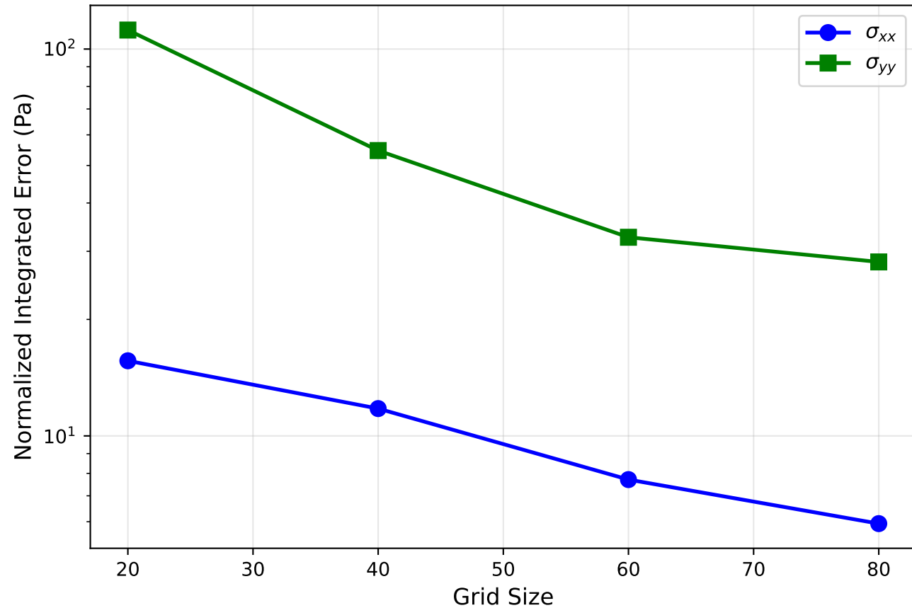
Normalized Integrated Error by Stress Component
