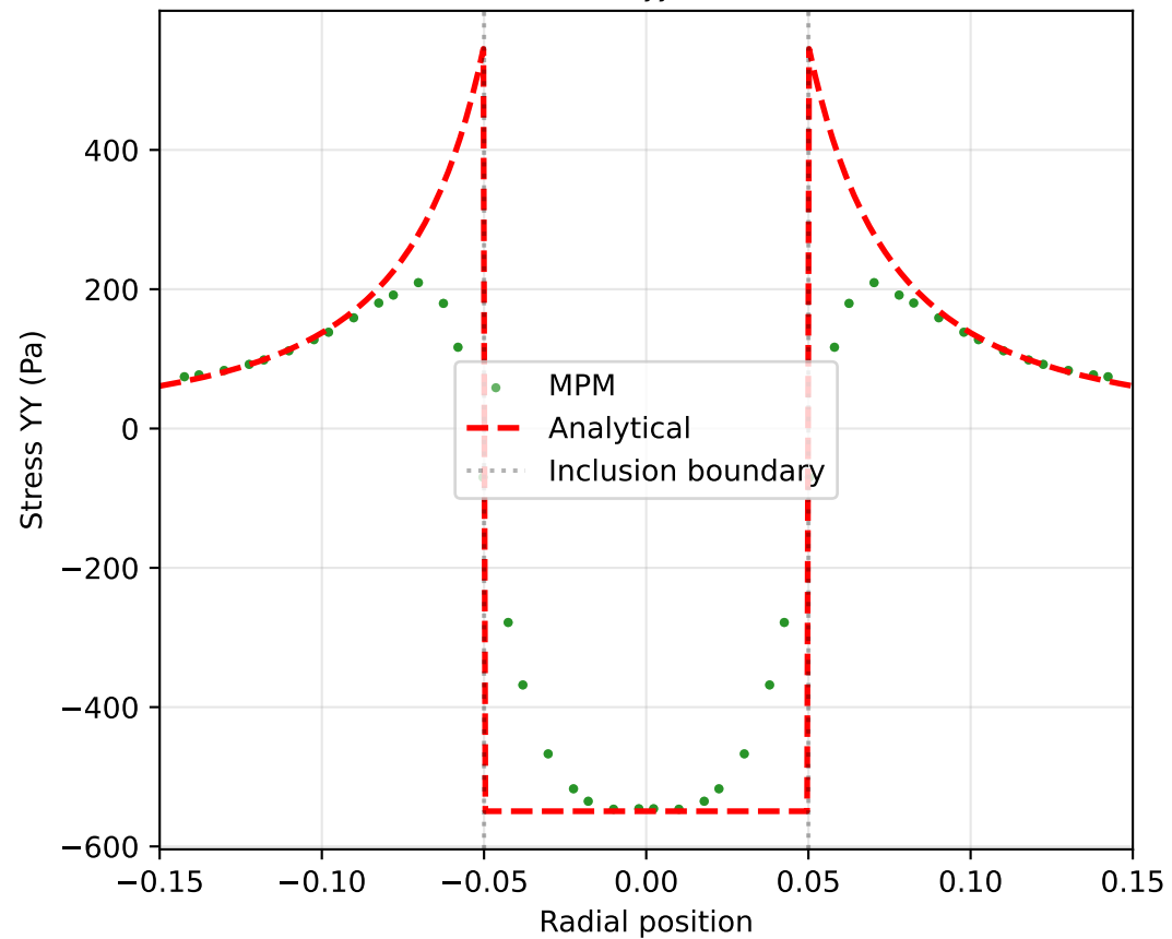
Radial Stress \sigma_{yy} (Grid 20x20)
