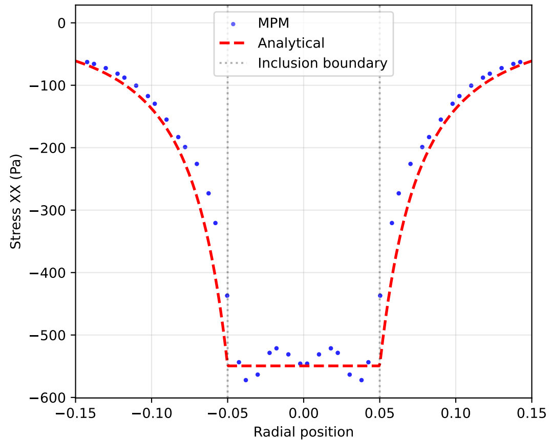
Transverse Stress \sigma_{xx} (Grid 20x20)
