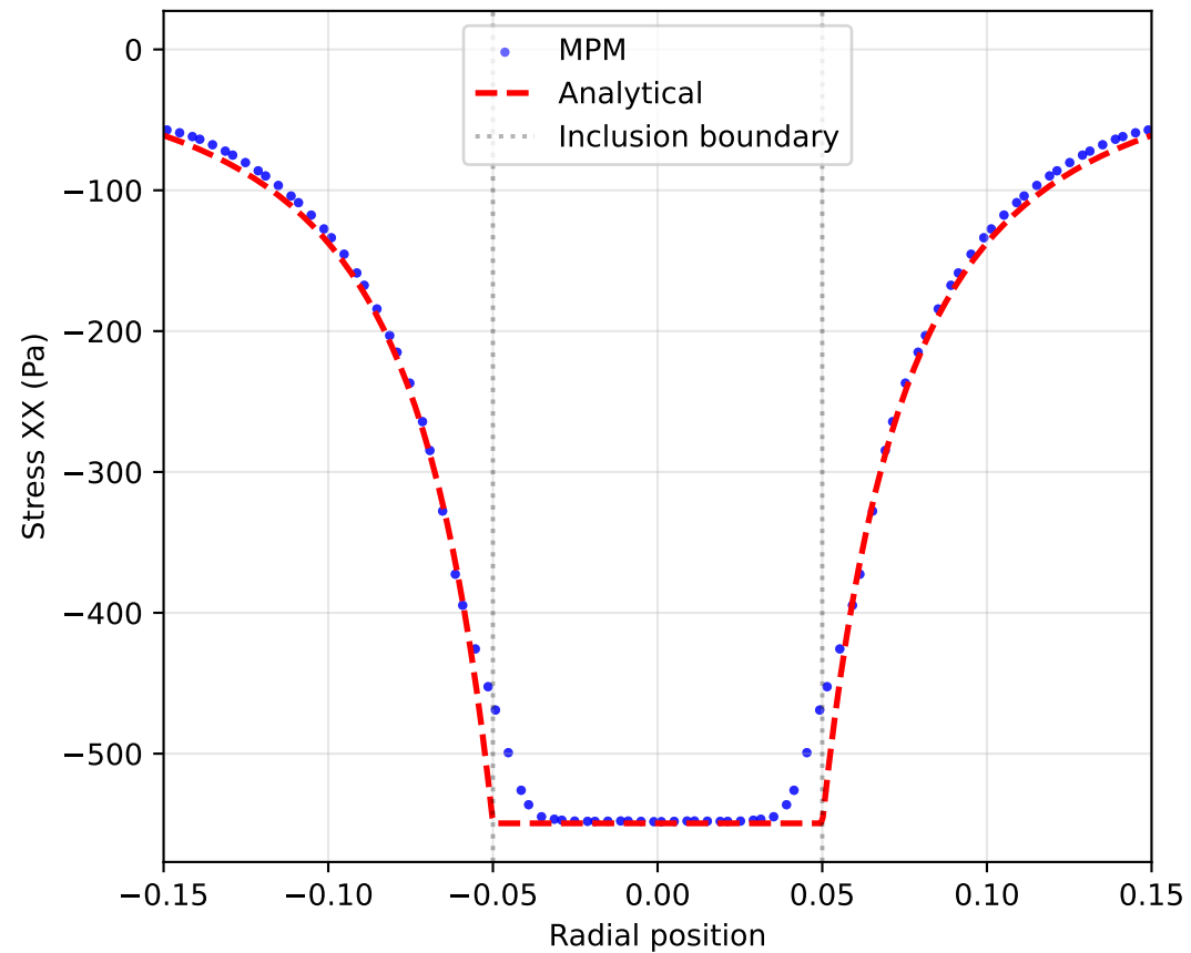
Transverse Stress \sigma_{xx} (Grid 40x40)
