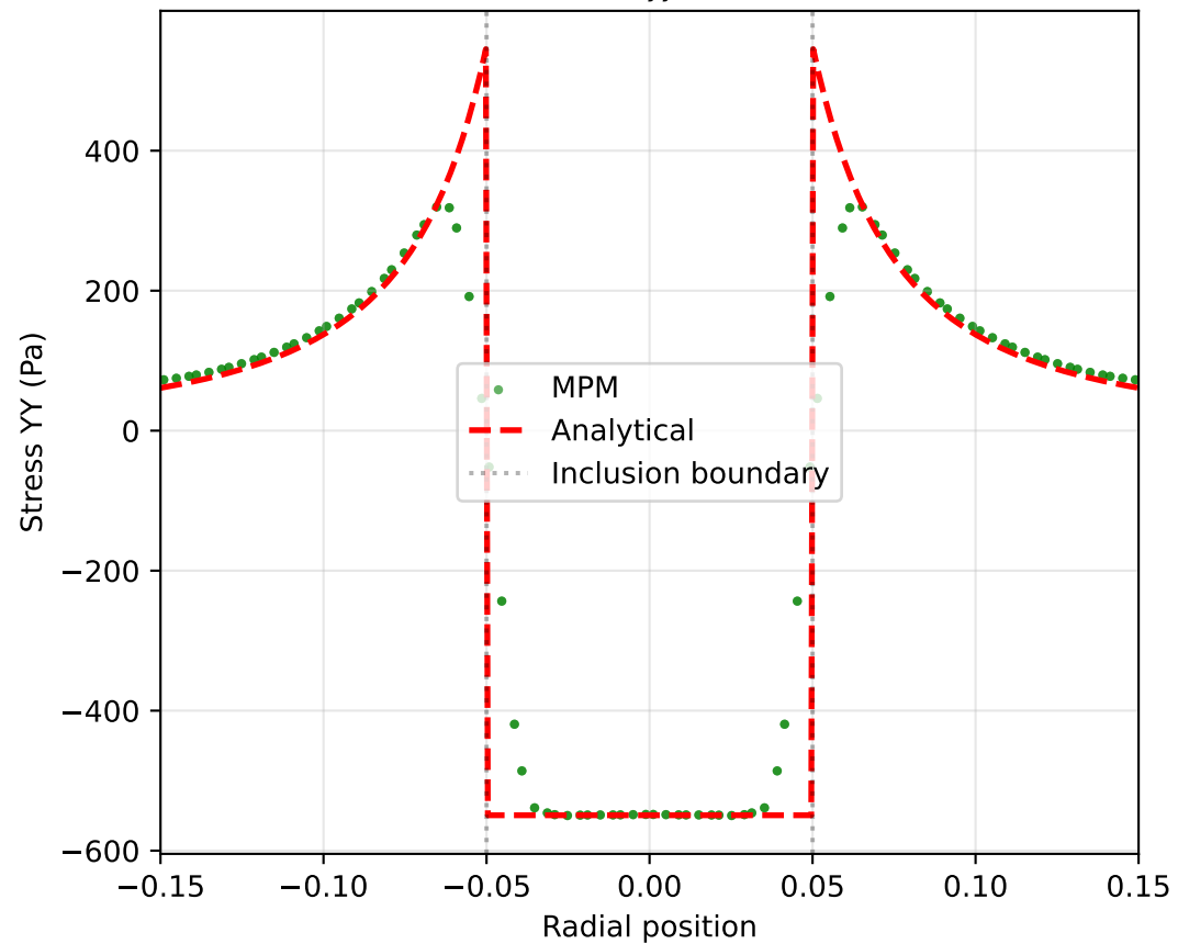
Radial Stress \sigma_{yy} (Grid 40x40)
