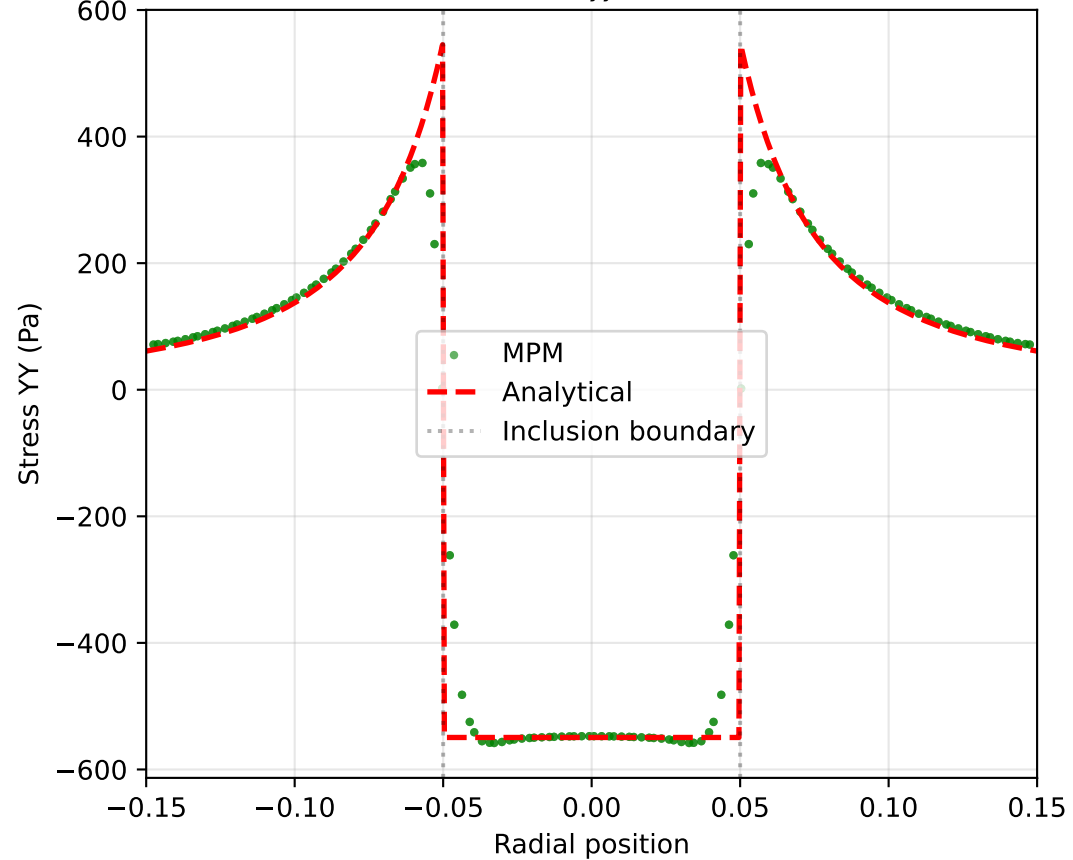
Radial Stress \sigma_{yy} (Grid 60x60)
