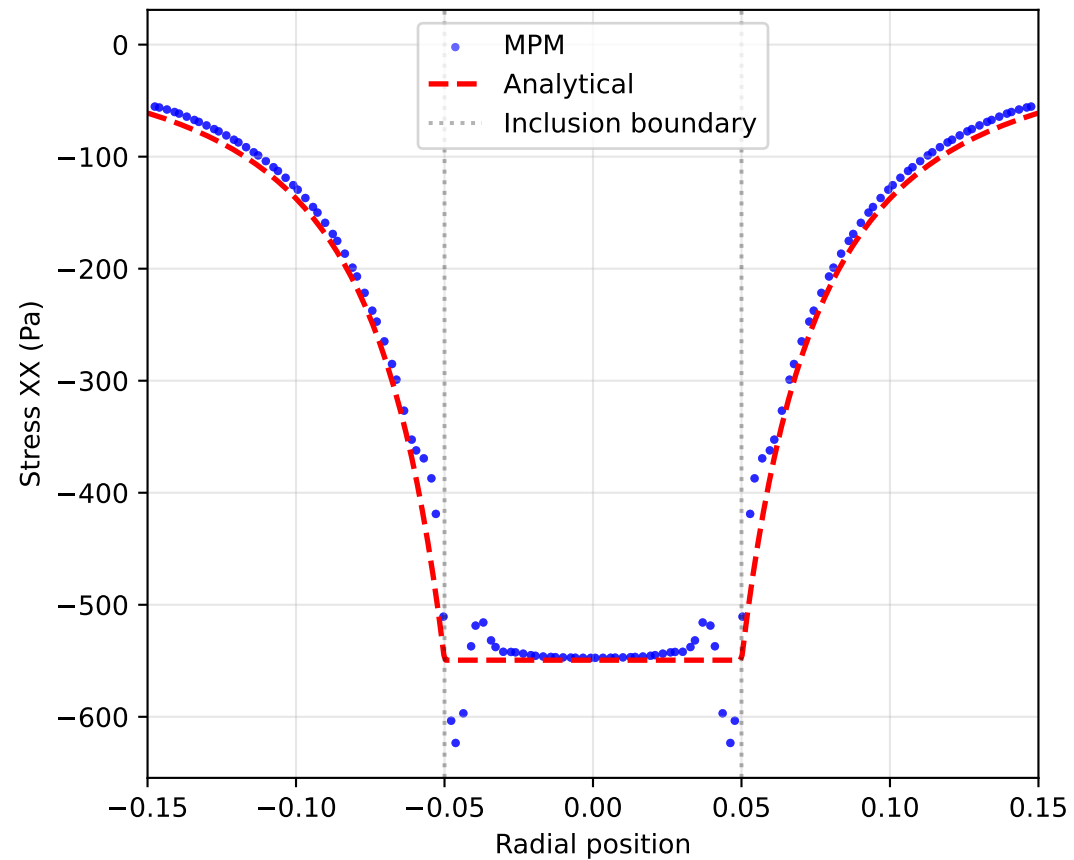
Transverse Stress \sigma_{xx} (Grid 60x60)
