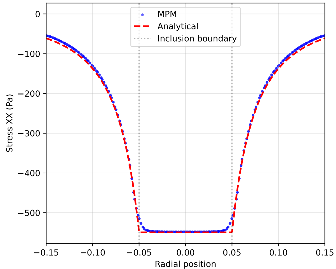
Transverse Stress \sigma_{xx} (Grid 80x80)
