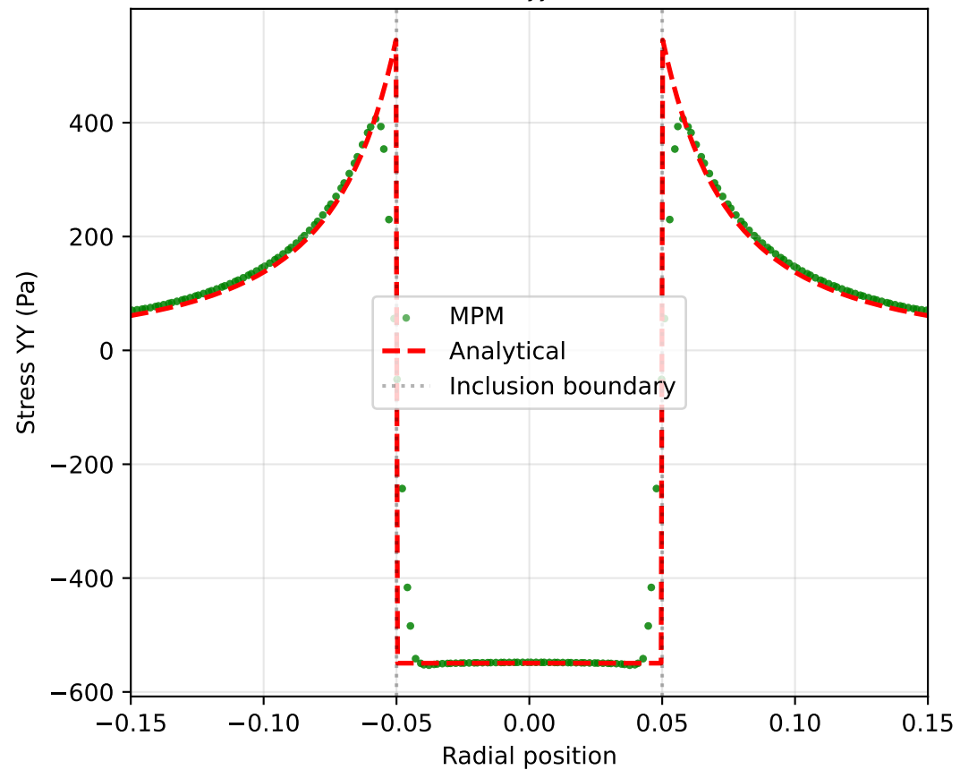
Radial Stress \sigma_{yy} (Grid 80x80)
