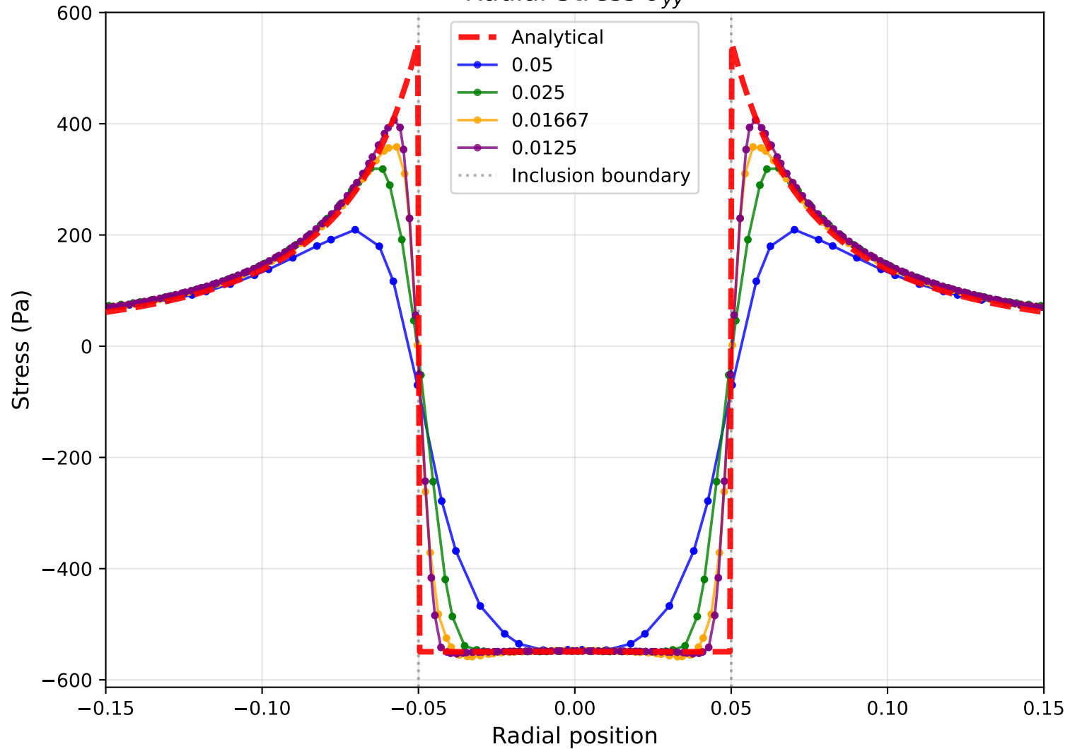
Radial Stress \sigma_{yy}
