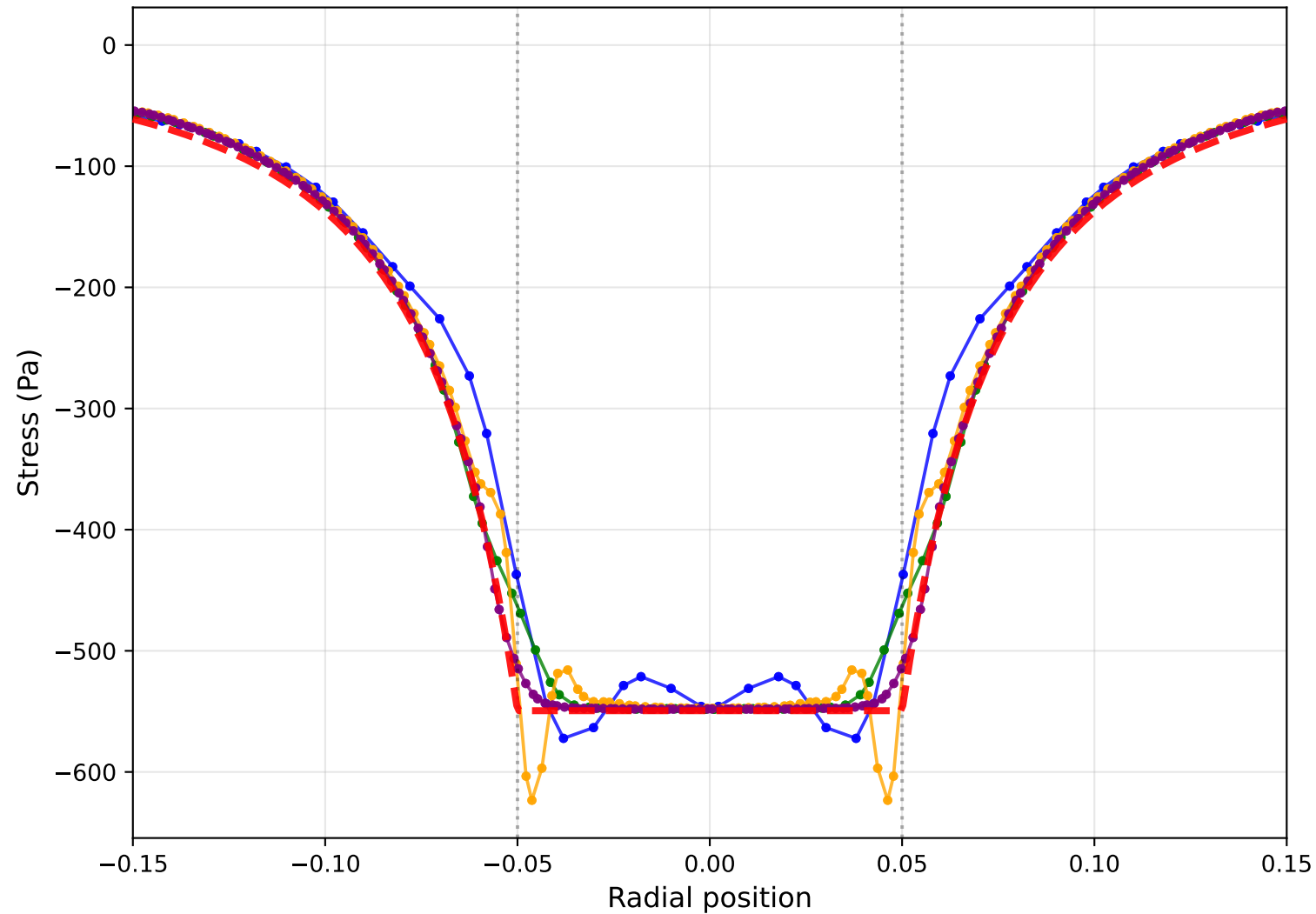
Transverse Stress \sigma_{xx}
