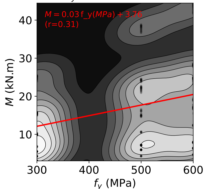
(h) f_y (MPa) vs. M (kN.m)
