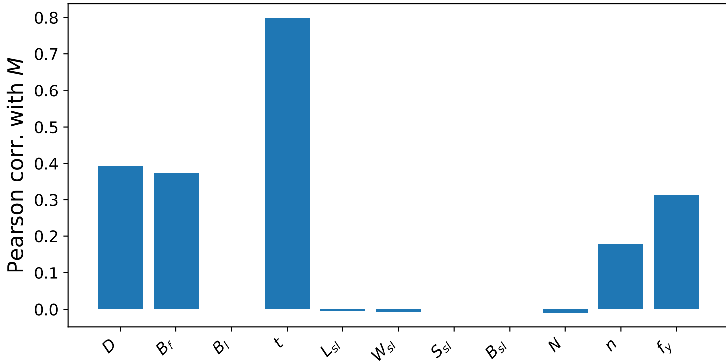
Feature-target correlation (Pearson)
