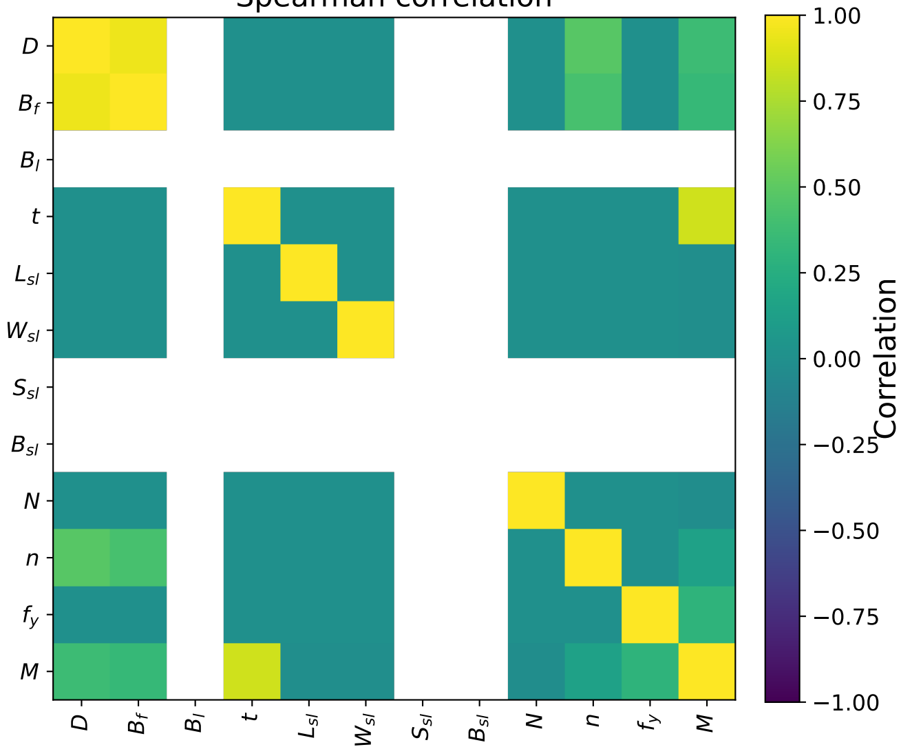
Spearman correlation
