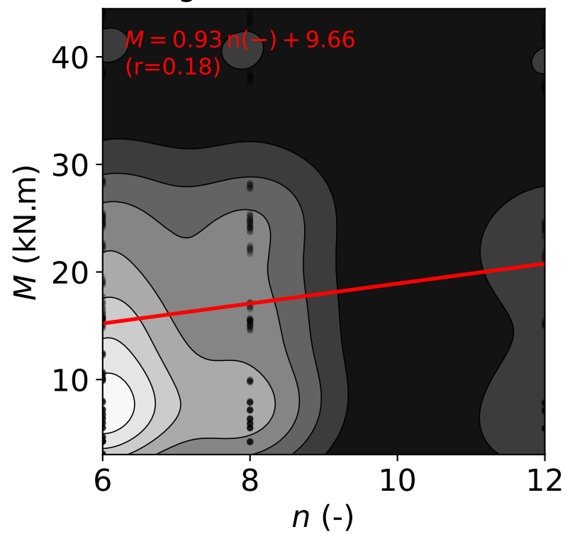
(g) n (-) vs. M (kN.m)
