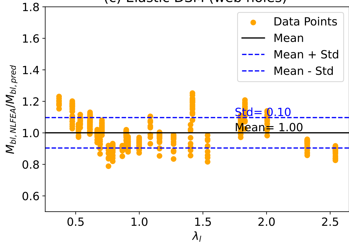
(c) Elastic DSM (web holes)
