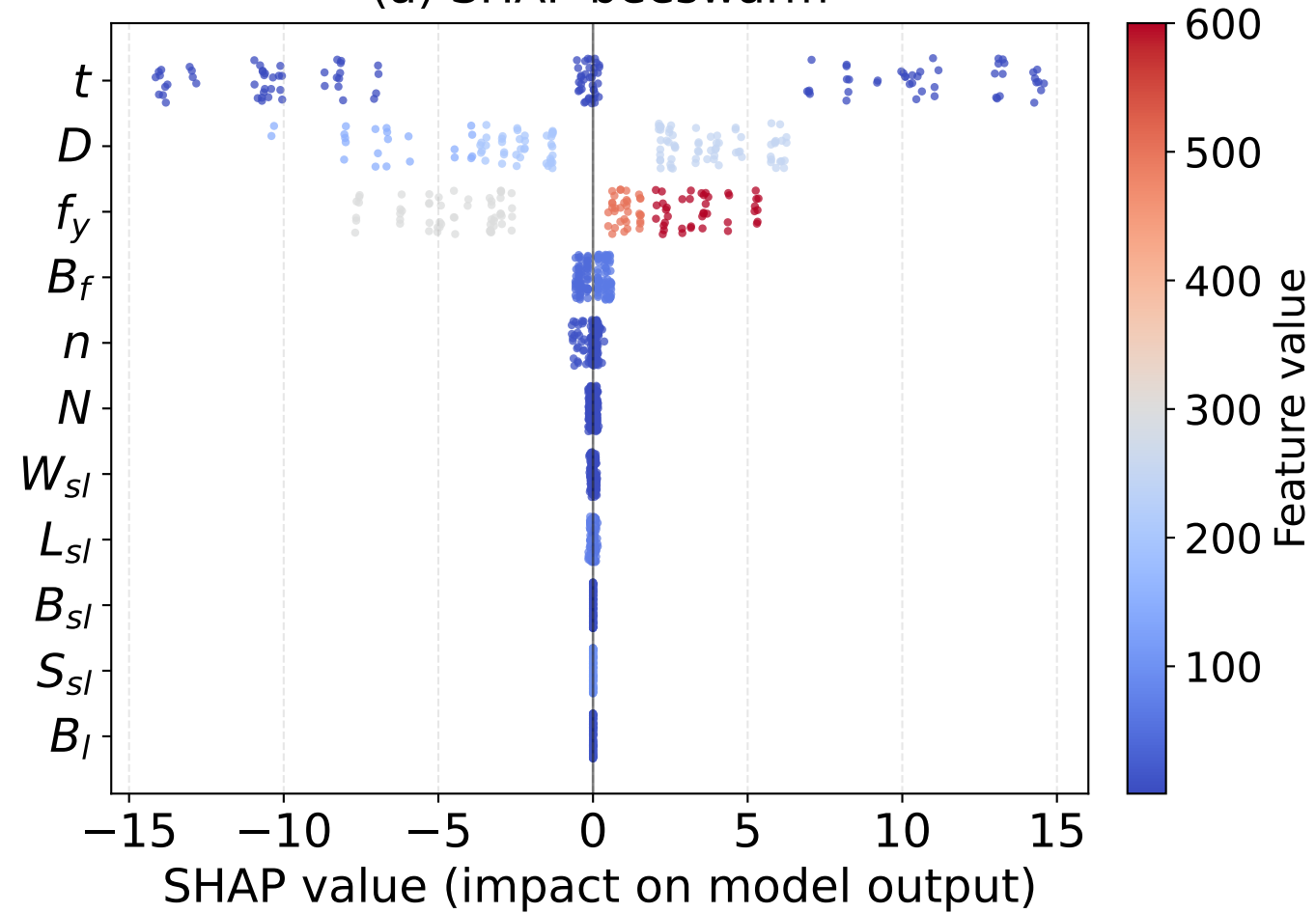
(a) SHAP beeswarm
