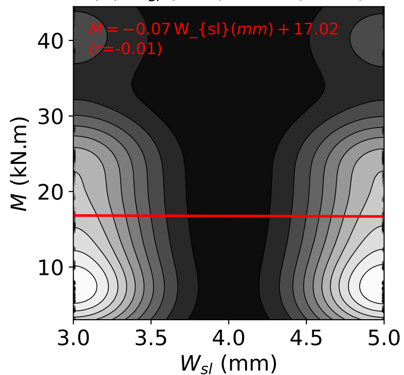
(e) W_{sl} (mm) vs. M (kN.m)
