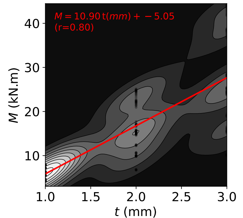
(c) t (mm) vs. M (kN.m)
