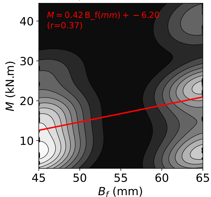
(b) B_f (mm) vs. M (kN.m)
