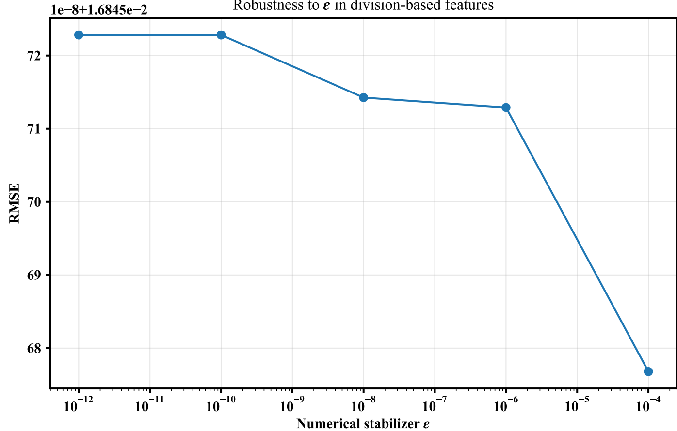
Robustness to \epsilon in division-based features
