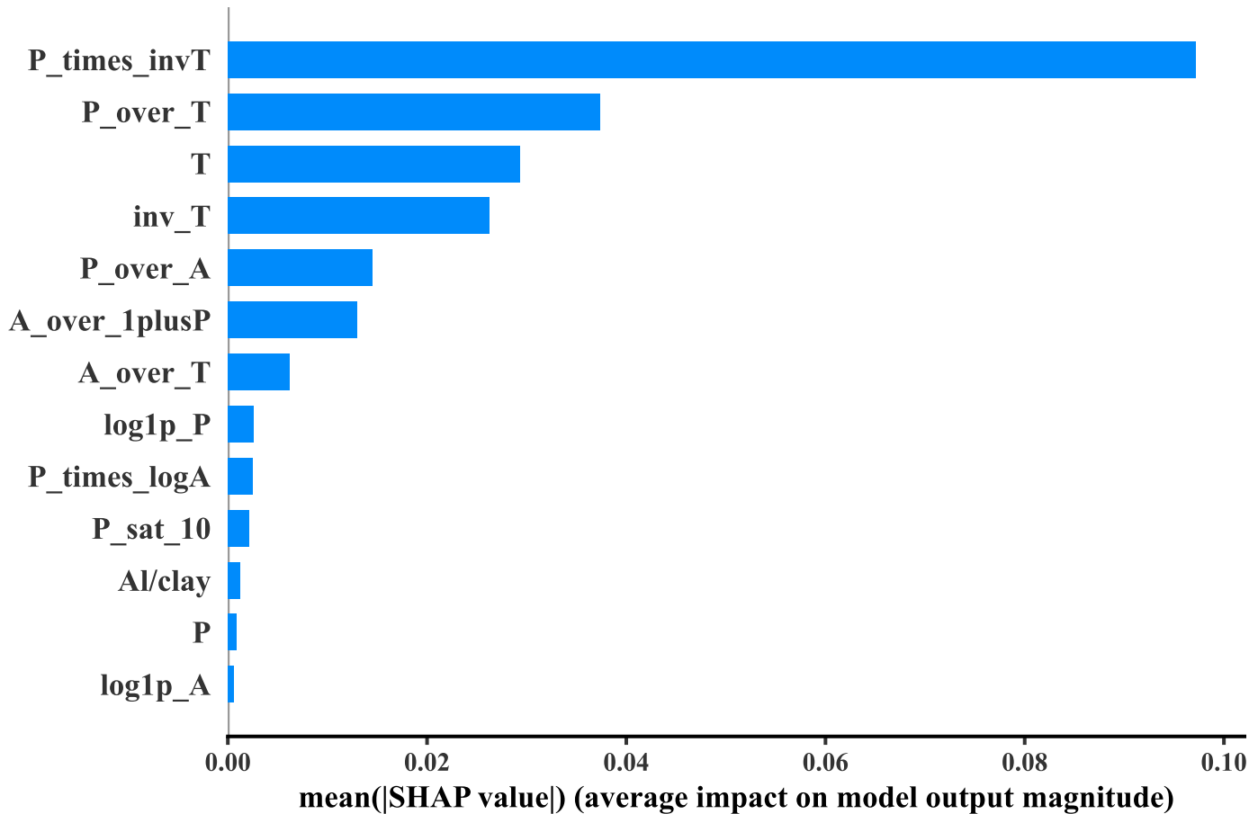
Mean absolute SHAP values: GBM
