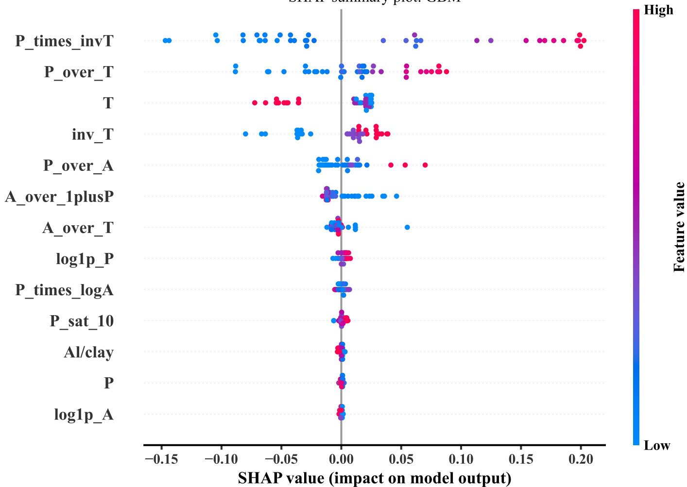
SHAP summary plot: GBM
