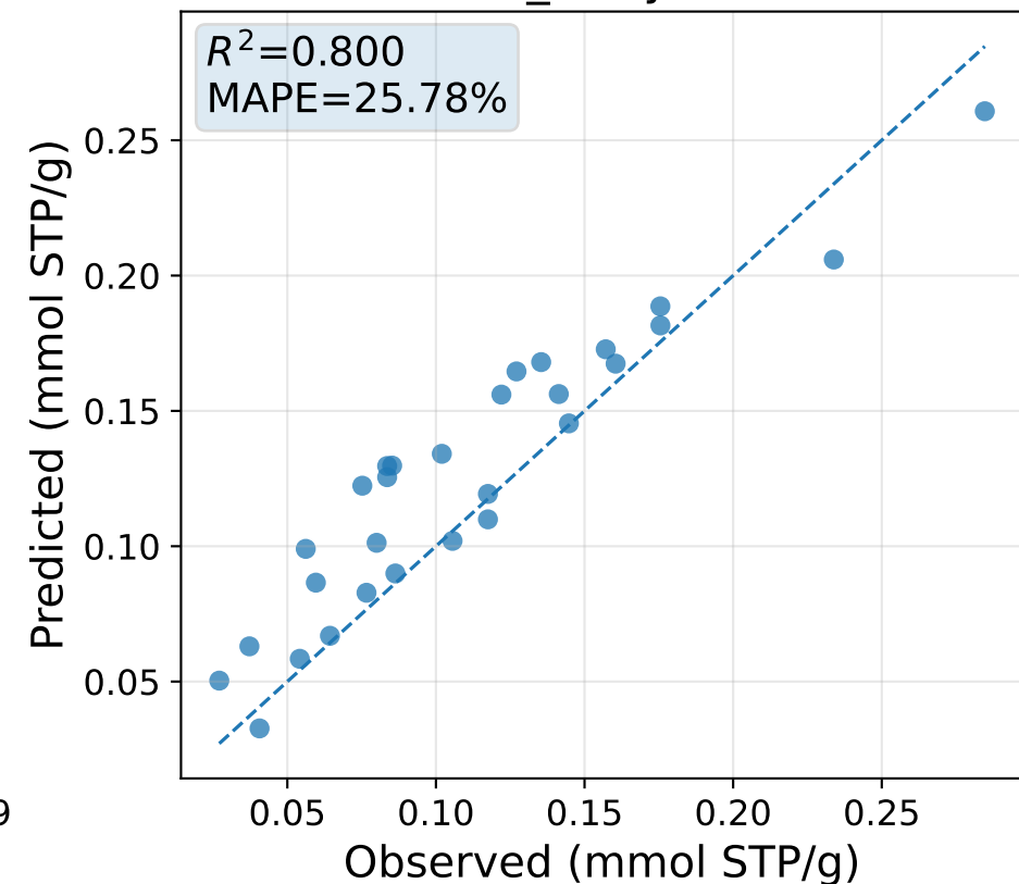
OOD_pressure_low PINN_PI-HySPAC
