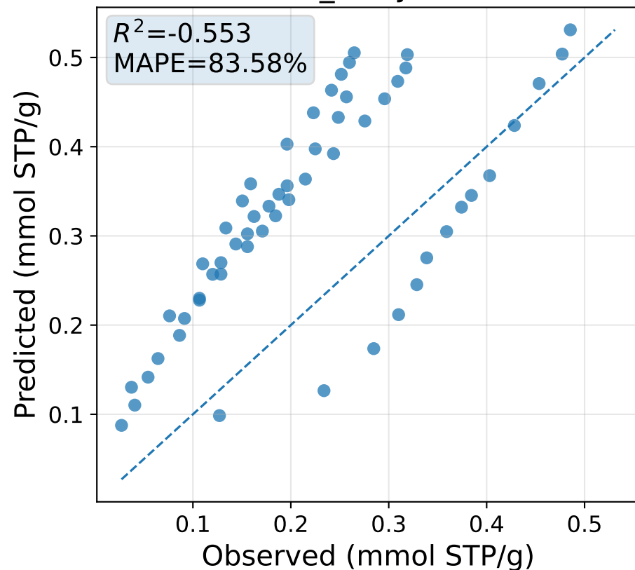
OOD_temp_max_group PINN_PI-HySPAC
