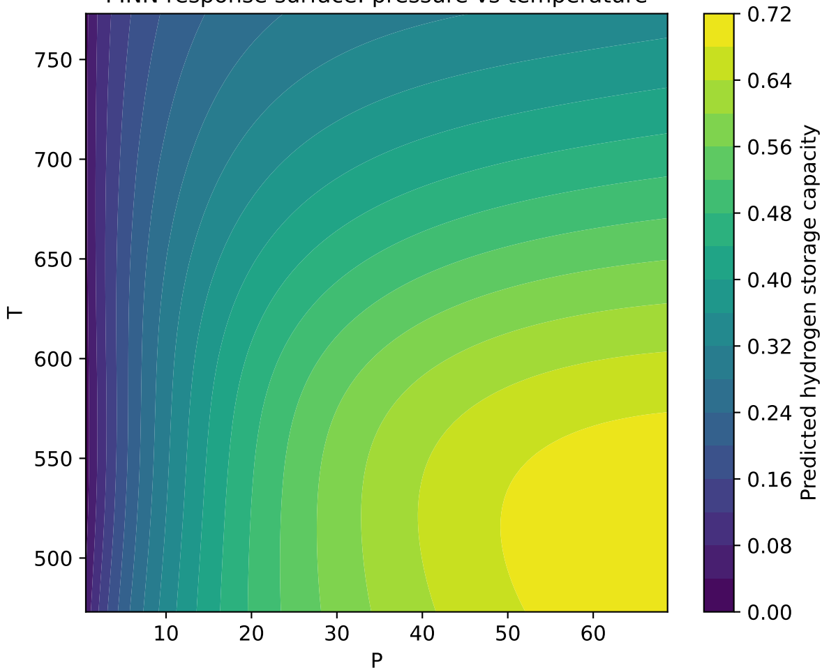
PINN response surface: pressure vs temperature
