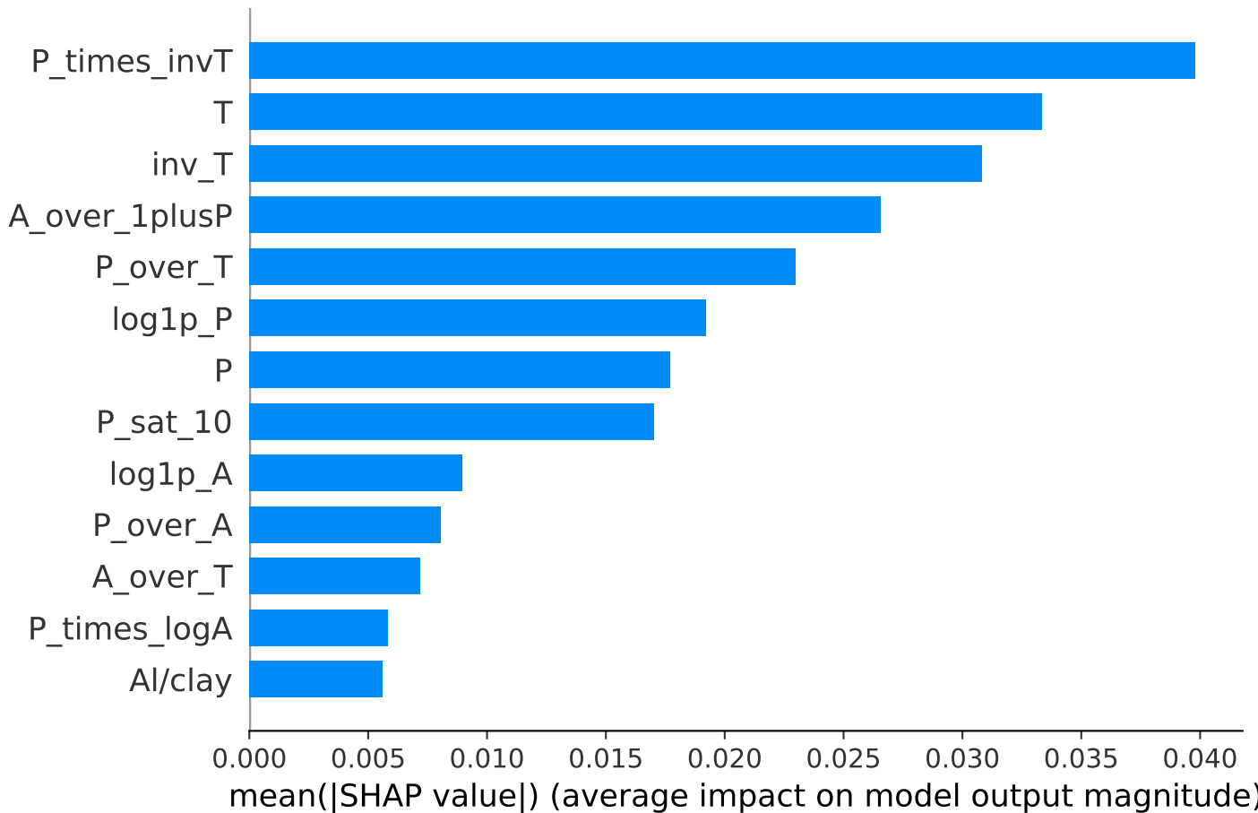
Mean absolute SHAP values: CatBoost
