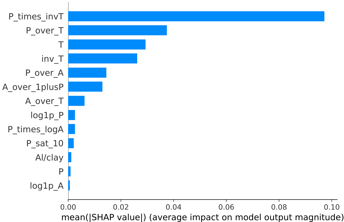
Mean absolute SHAP values: GBM
