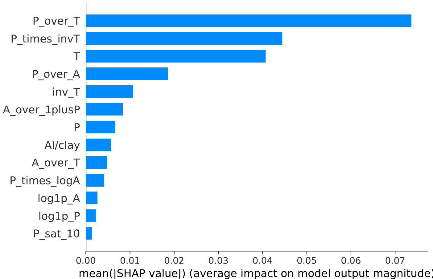
Mean absolute SHAP values: XGBoost
