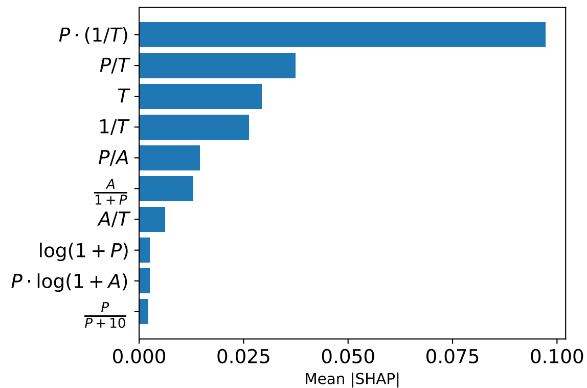
XGBoost
