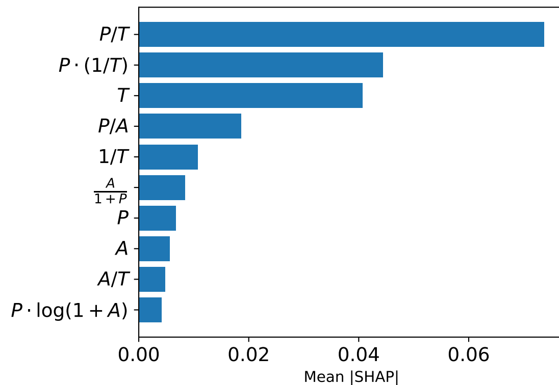
XGBoost
