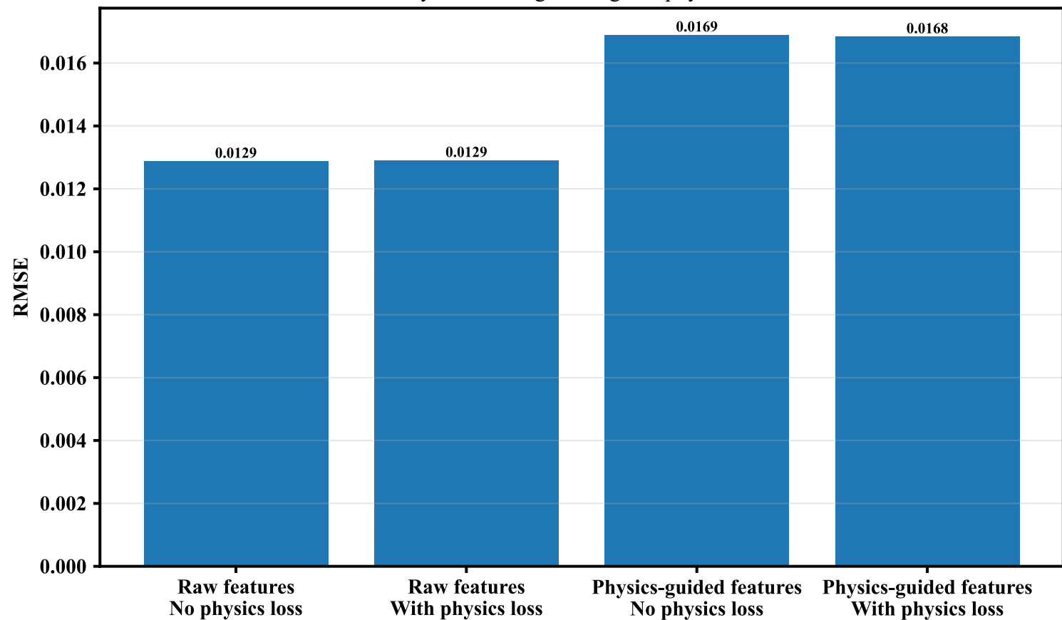
Ablation study: feature engineering and physics-informed loss
