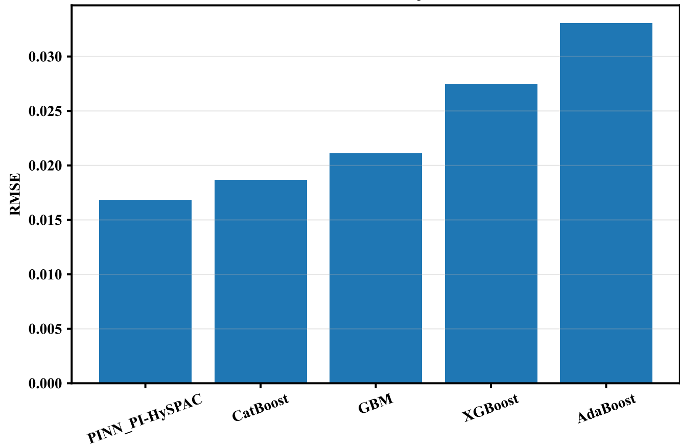
IID test RMSE comparison
