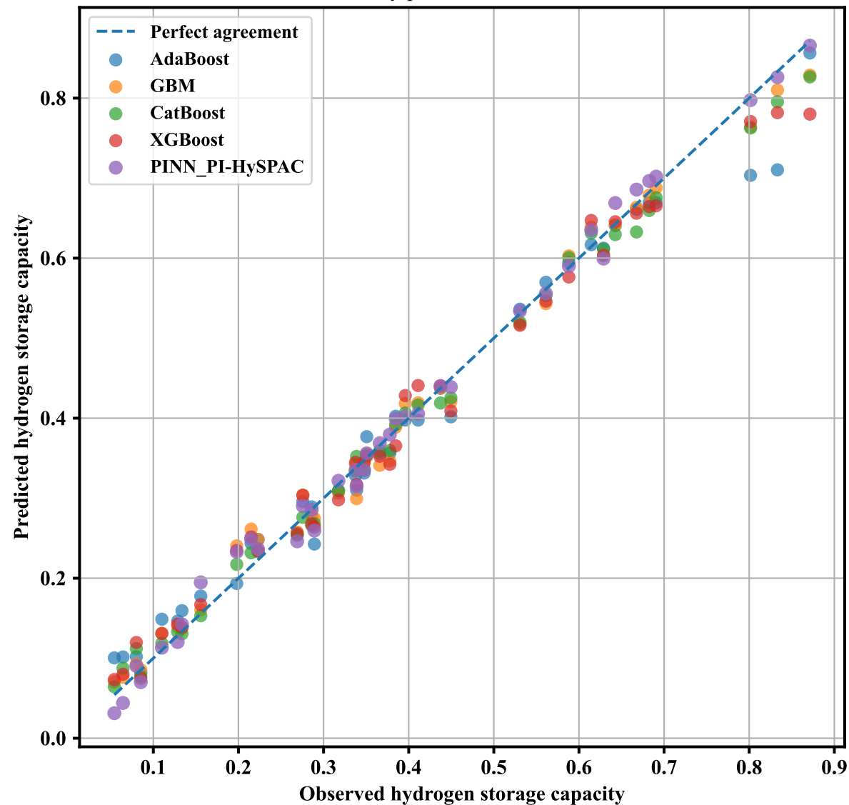
Parity plot on IID test set
