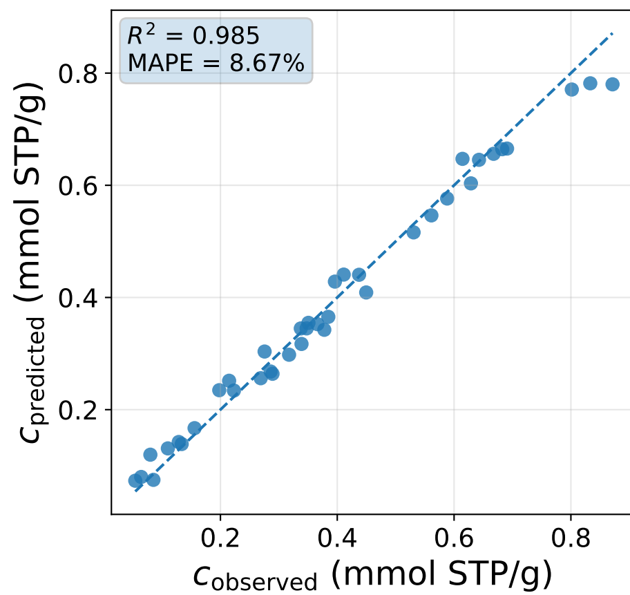
XGBoost
