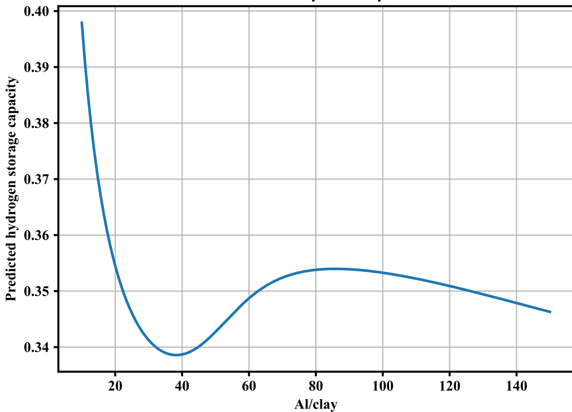
PINN sensitivity to Al/clay ratio
