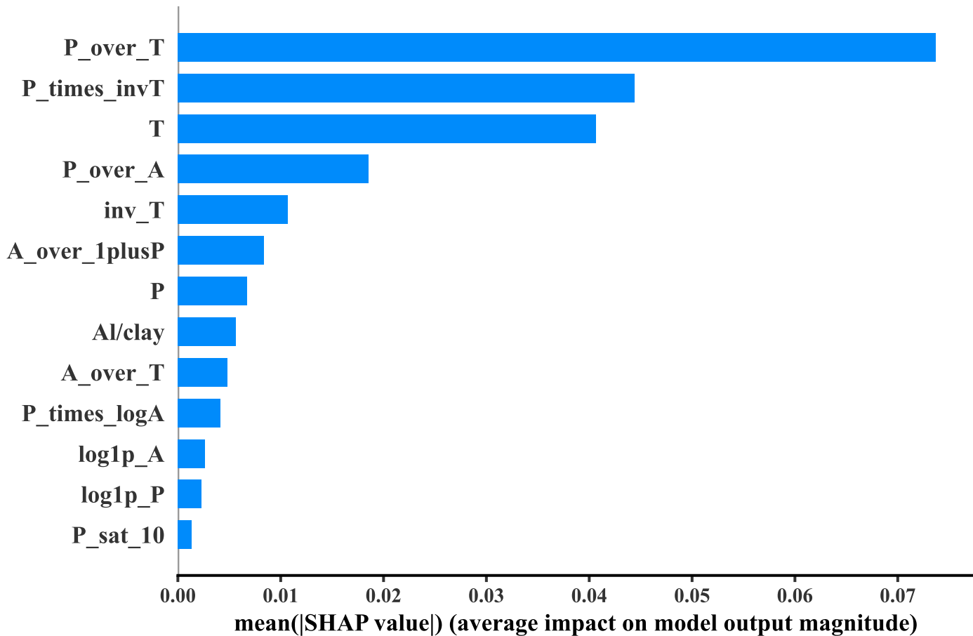
Mean absolute SHAP values: XGBoost
