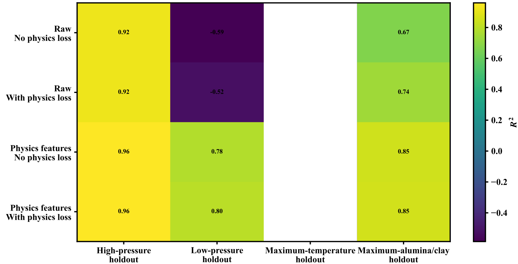
Out-of-distribution ablation and failure modes
