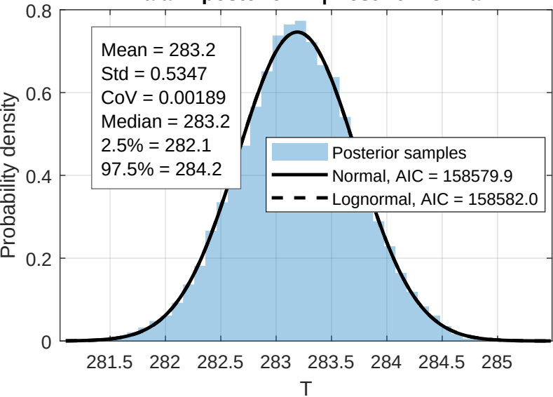
malami posterior: T | Best fit: Normal
