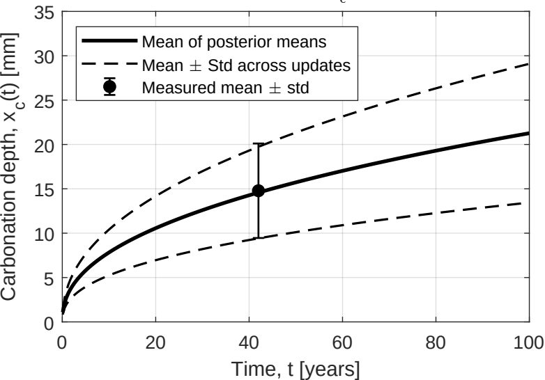
(c) fib Bulletin 34, \sigma_{\epsilon} = 2.5 mm
