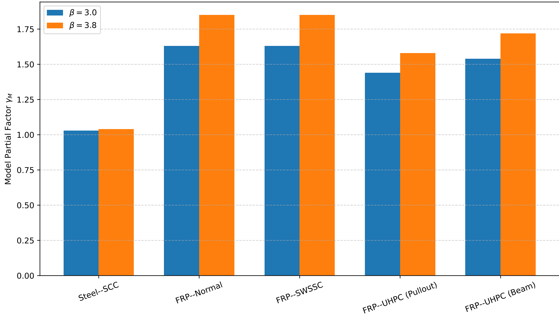
Calibrated Model Partial Factors for Different Reliability Indices
