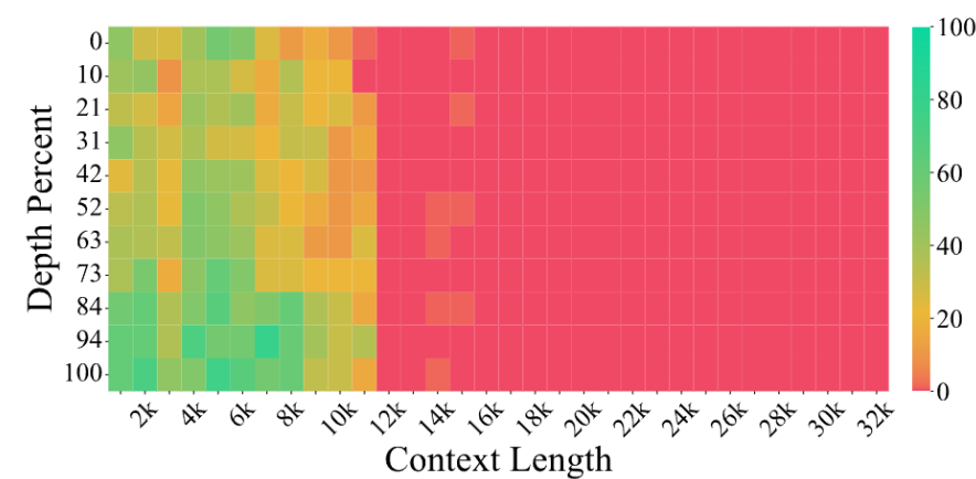
3B-8K llama based model의 NIAH [3]
