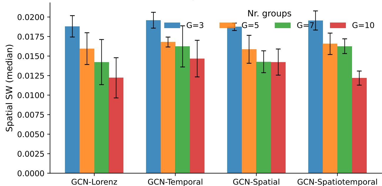
Xian — Spatial SW (median)
