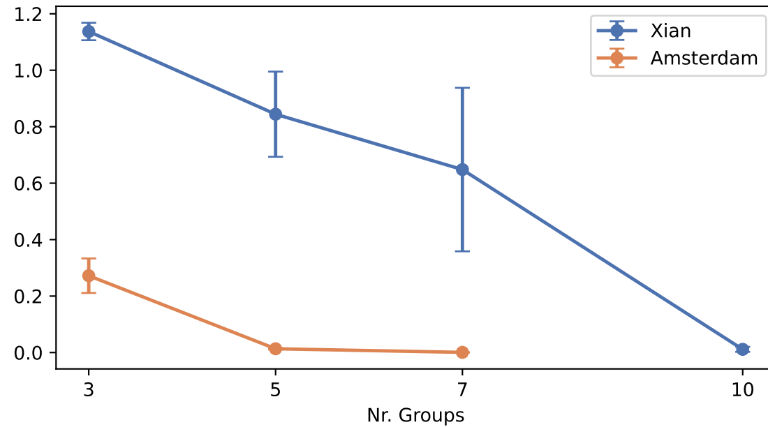
Hypervolume
