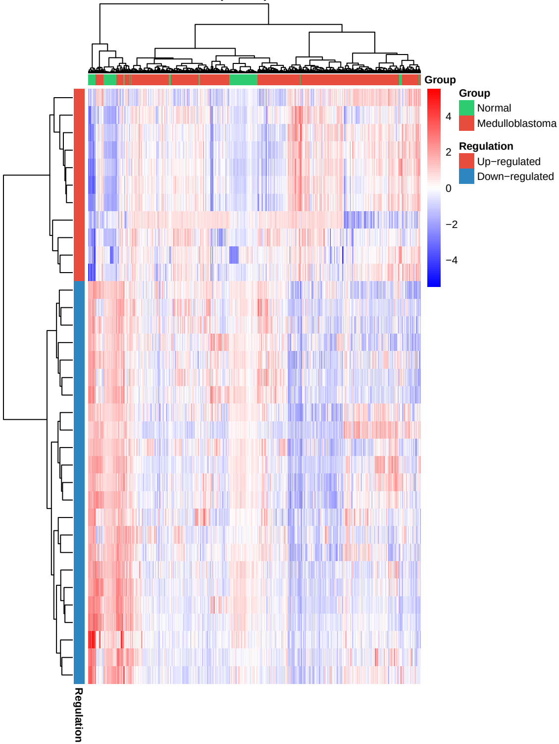
Heatmap of Top 100 DEGs
