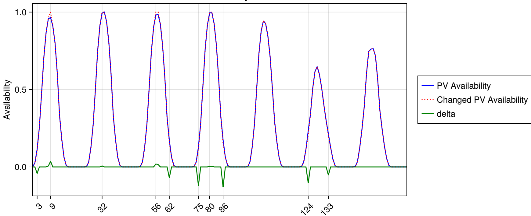
PV Availability
