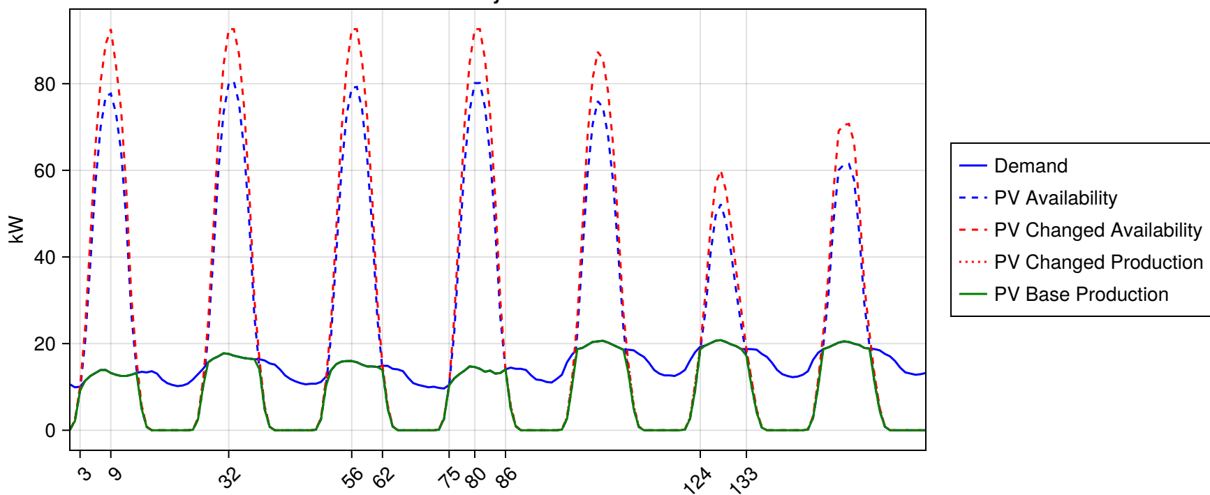
Electricity Demand
