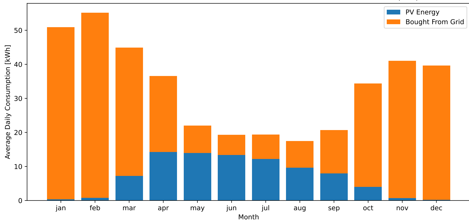
AVERAGE DAILY CONSUMPTION: SELF-PRODUCED OR BOUGHT FROM THE GRID (DURING THE DAYTIME)
