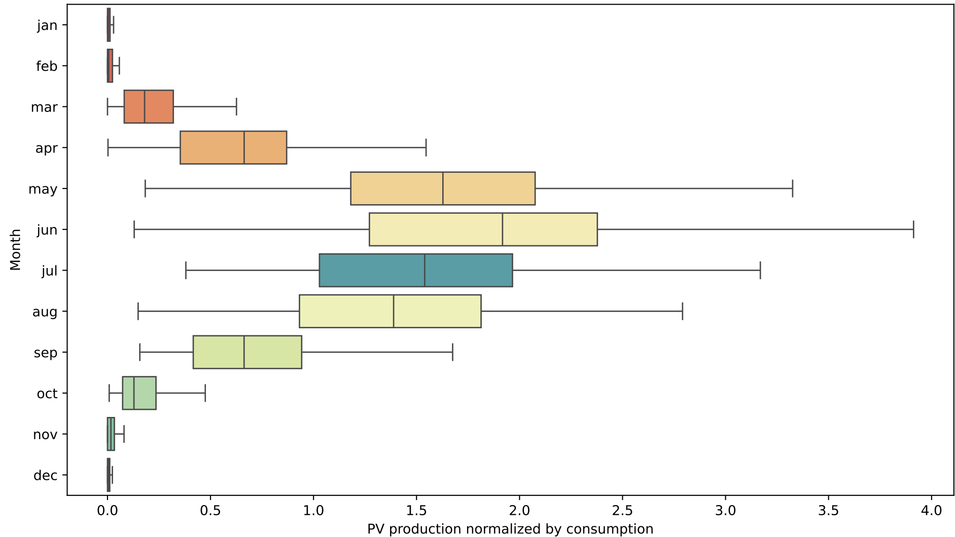
PV PRODUCTION NORMALIZED BY CONSUMPTION
