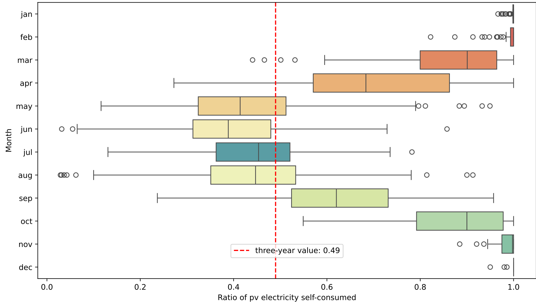
PV SELF CONSUMPTION RATIO DISTRIBUTION BY MONTH
