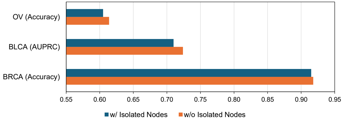
Figure. Ablation study on the effect of handling isolated nodes by connecting them to the most similar patient in MAGNET.
