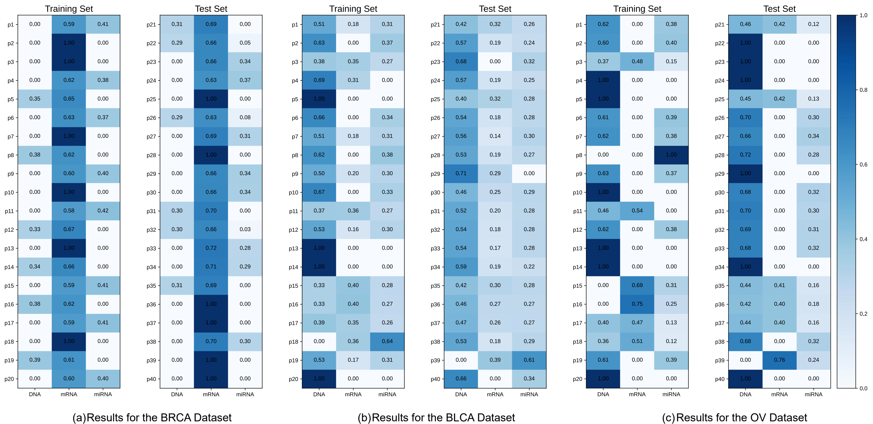
Figure. Attention weights learned by MAGNET for 20 selected patients across modalities in training and test sets for each dataset.
