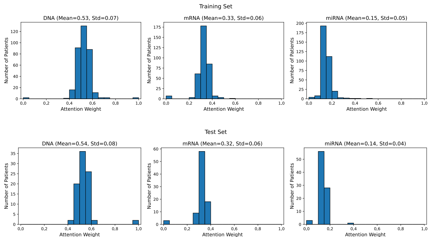
Figure. Distribution of attention weights across modalities for the BLCA dataset in training and test sets. Mean and standard deviation are reported for each modality.
