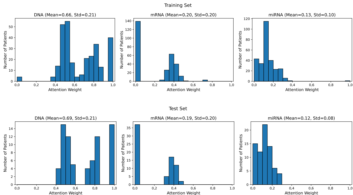
Figure. Distribution of attention weights across modalities for the OV dataset in training and test sets. Mean and standard deviation are reported for each modality.
