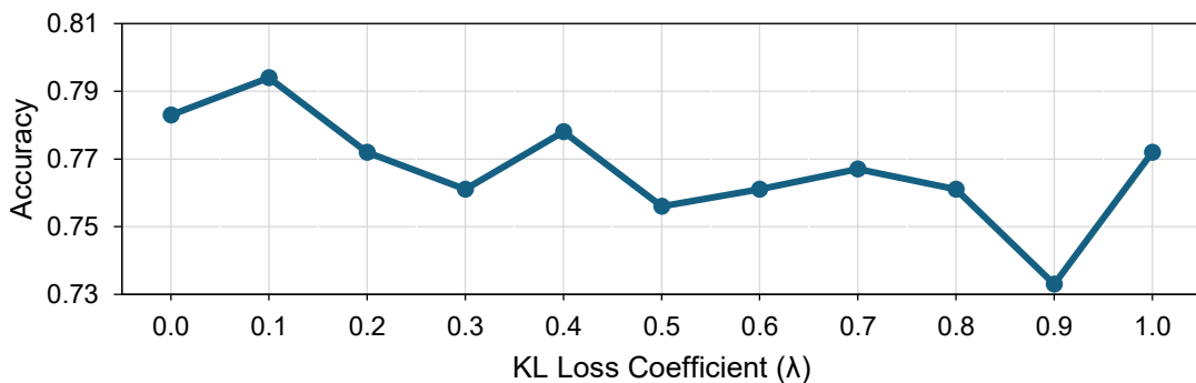
Figure. Impact of the KL loss coefficient ( \lambda ) on MAGNET performance over validation sets across datasets.
