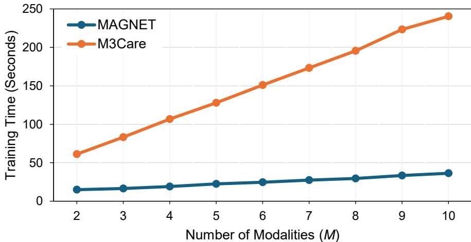
Figure. Training time comparison between MAGNET and M3Care on a synthetic dataset with an increasing number of modalities ( M = 2 - 10 ).
