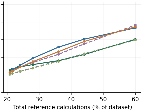
Transition1x
