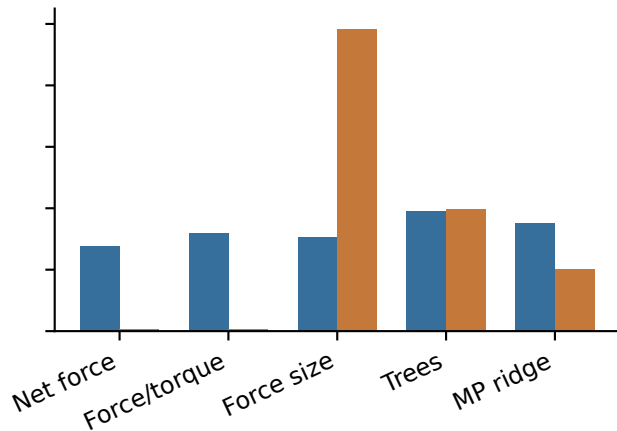
Transition1x
