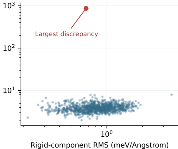
Transition1x
