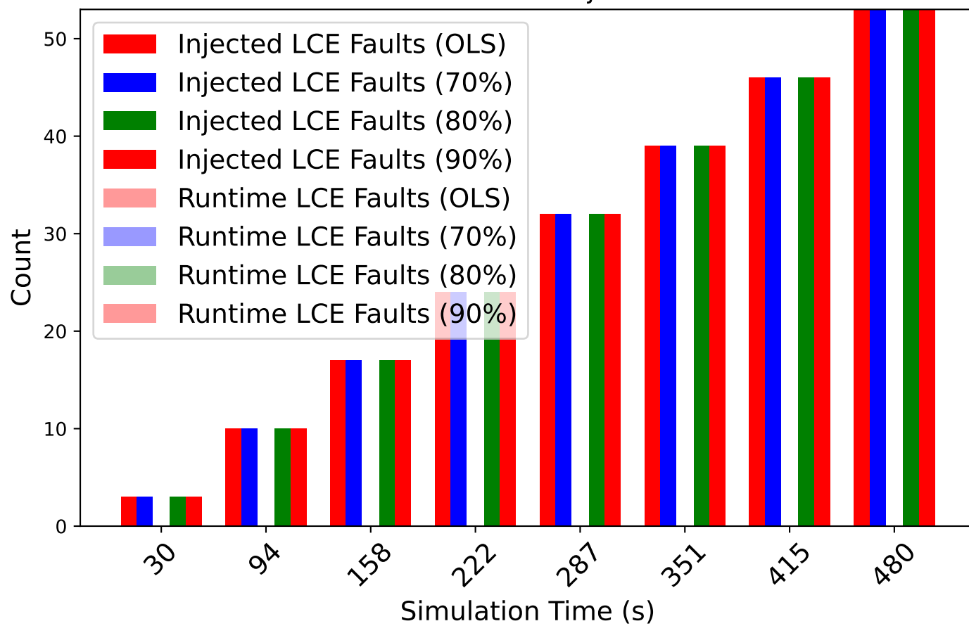
Runtime LCE Faults and Injected LCE Faults
