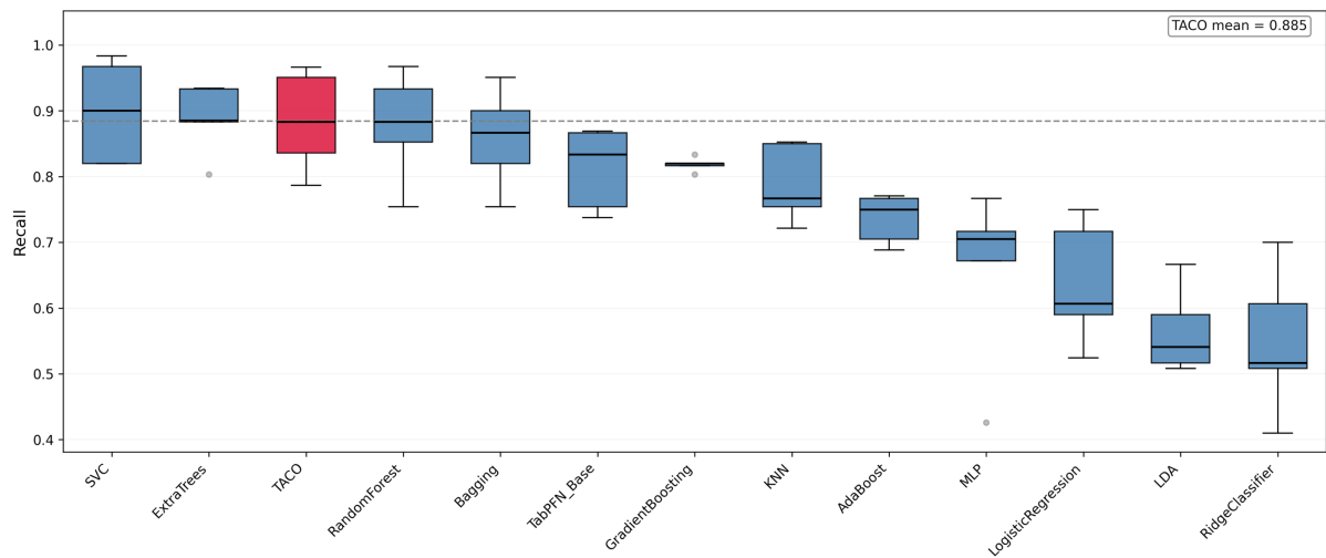
TACO Comparison Recall Sorted by Median:
