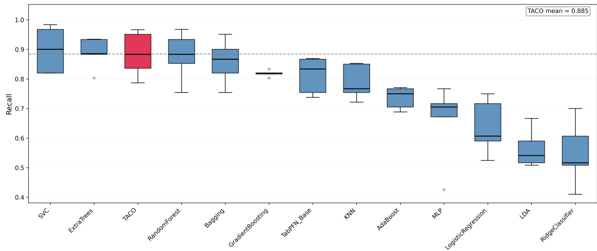
TACO Comparison Recall Sorted by Mean:
