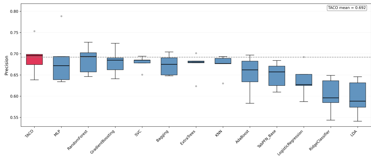
TACO Comparison Precision Sorted by Mean:
