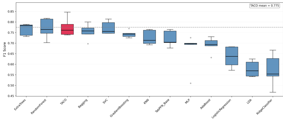
TACO Comparison F1 Score Sorted by Median:
