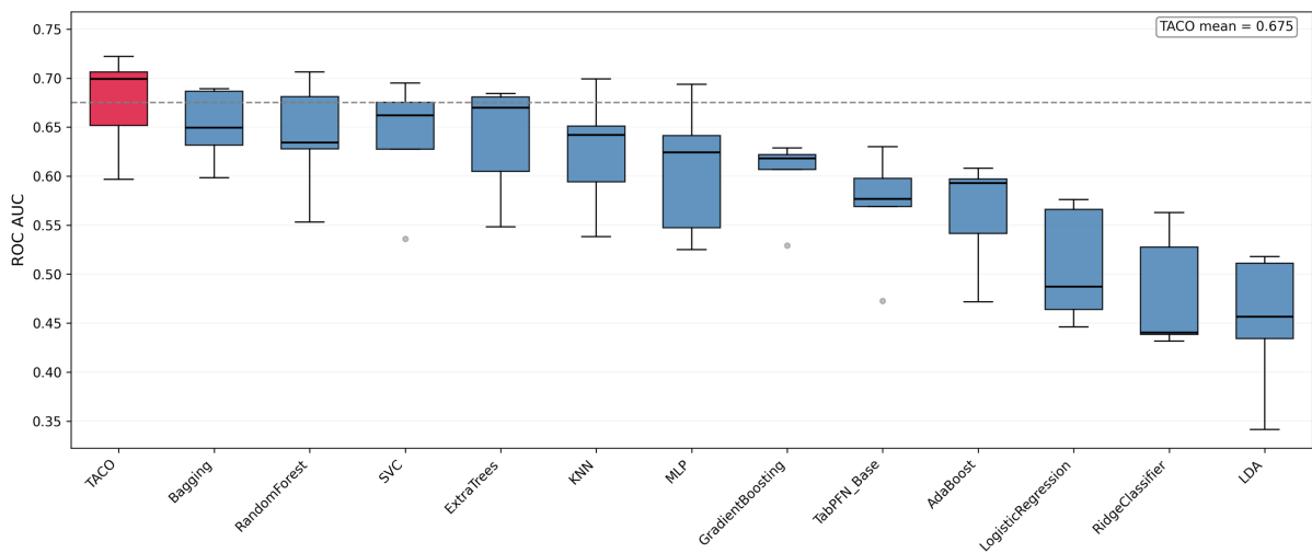
TACO Comparison ROC-AUC Sorted by Mean:
