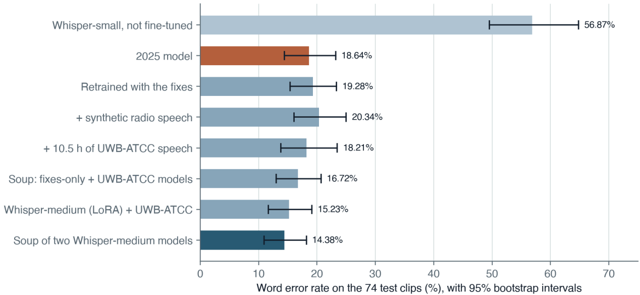
Figure 2. Word error rate on the 74 test clips. The dark bar is the model selected on validation.
