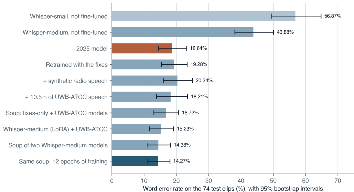
Figure 2. Word error rate on the 74 test clips. The dark bar is the model selected on validation.
