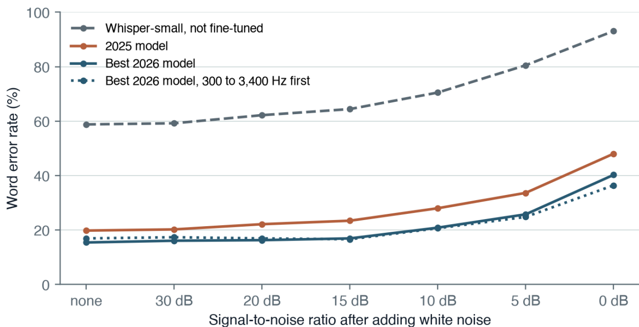
Figure 4. Word error rate on the 74 test clips as white noise is added. Greedy decoding with repetition guards. The filtered clips receive about 2 dB less noise at each nominal ratio, because the filter lowers the clip power the noise is set from.
