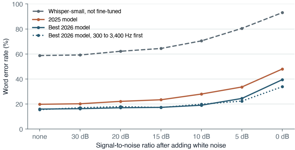
Figure 4. Word error rate on the 74 test clips as white noise is added. Greedy decoding with repetition guards. The filtered clips receive about 2 dB less noise at each nominal ratio, because the filter lowers the clip power the noise is set from.
