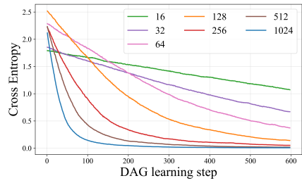
(b) Classification
